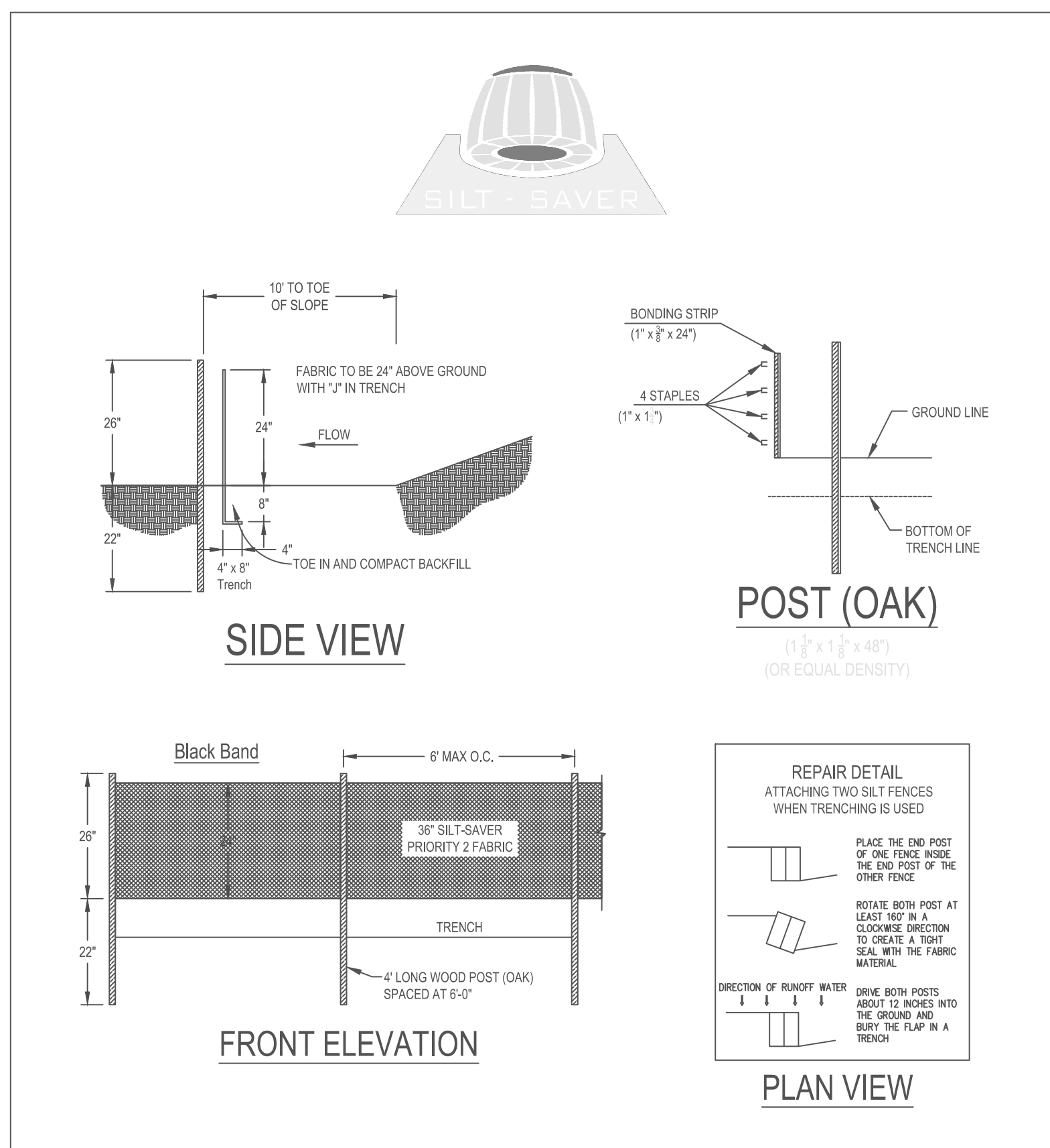
2 BELTED SILT RETENTION FENCE PRIORITY 2 (BSRF2) Z9949C NOT TO SCALE
